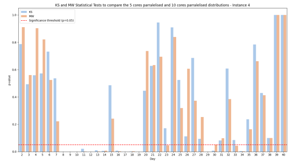
Fig. 29. Statistical tests to compare the 5 and 10 cores distribution - Instance 4
