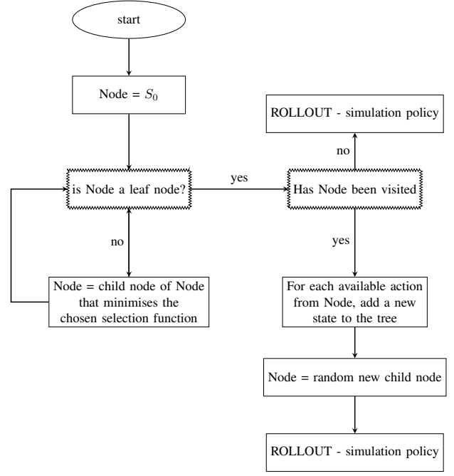
Fig. 14. Flow MCTS
